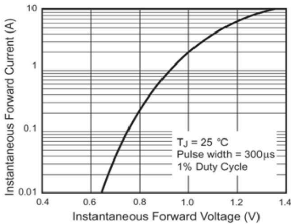
Figure 3. Typical Forward Characteristics Per Leg
