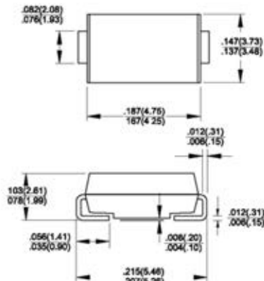
DO-214AA (SMB)
