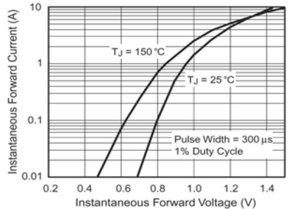
Figure 3. Typical Forward Voltage Characteristics Per Leg
