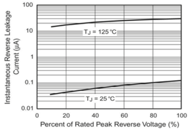
Figure 4. Typical Reverse Leakage Characteristics Per Leg
