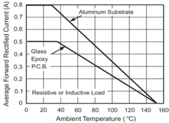
Figure 1. Derating Curve for Output Rectified Current
