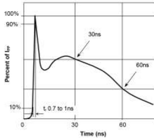
Fig.4 Pulse Waveform-ESD(IEC61000-4-2)
