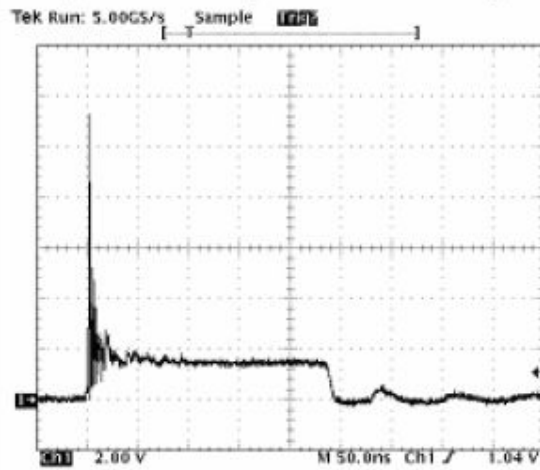
Figure 3. ESD Clamping (8kV Contact per IEC 61000-4-2)
