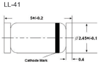
Glass case MELF Dimensions in mm
