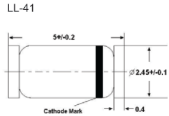
Glass case MELF Dimensions in mm
