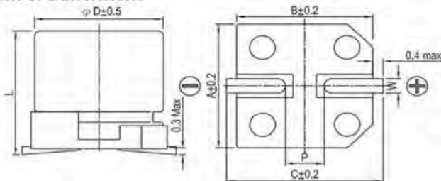
Lead Spacing and Diameter
