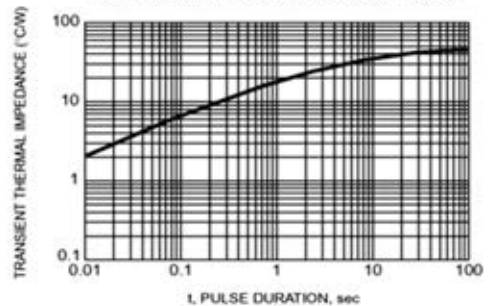
FIG. 6 - TYPICAL TRANSIENT THERMAL IMPEDANCE
