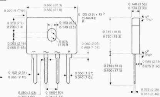
Package outline dimensions in inches (millimeters)
