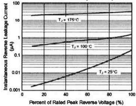
Fig. 4 – Typical Reverse Leakage Characteristics (MUR120)
