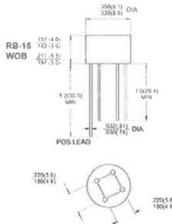
Package outline dimensions in inches (millimeters)
