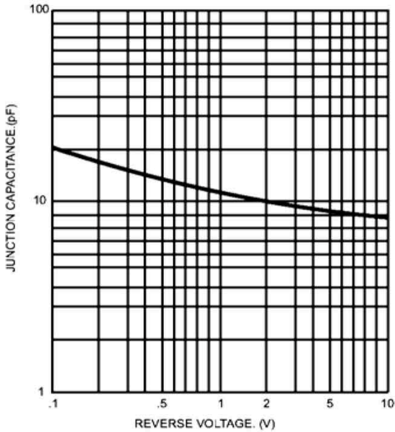
FIG.3- TYPICAL JUNCTION CAPACITANCE
