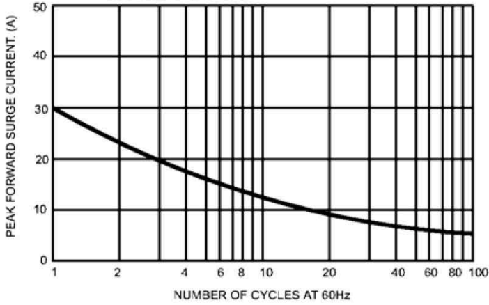
FIG.1- MAXIMUM NON-REPETITIVE FORWARD SURGE CURRENT
