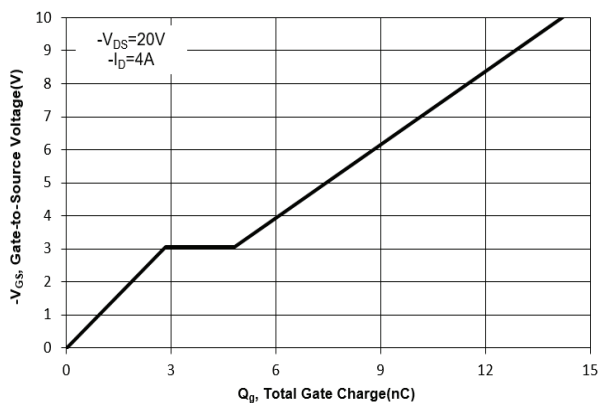
Fig. 11 Gate Charge
