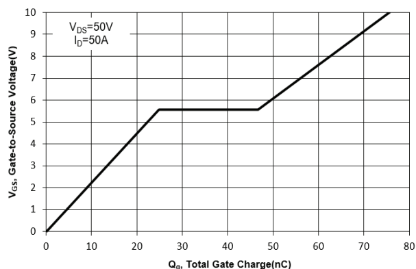
Fig. 11 Gate Charge
