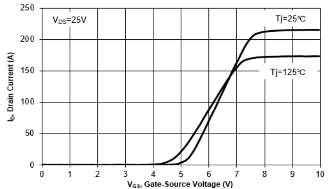
Fig. 2 Typical Transfer Characteristics
