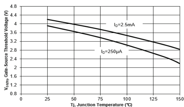
Fig. 10 Gate Threshold Variation vs. T_J
