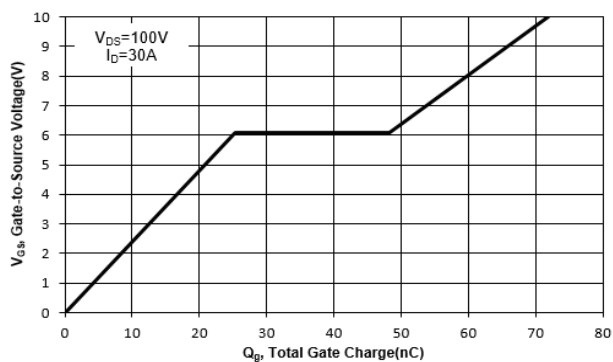
Fig. 11 Gate Charge
