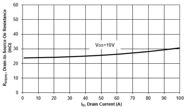
Fig. 3 on-Resistance vs. Drain Current
