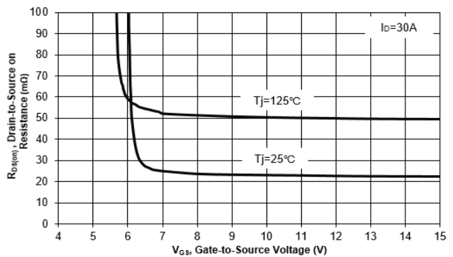
Fig. 4 on-Resistance vs. Gate to Source Voltage
