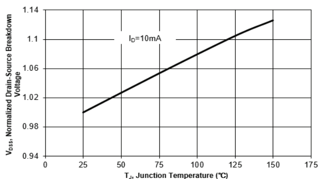
Fig. 9 V_{(BR)DSS} vs. Junction Temperature
