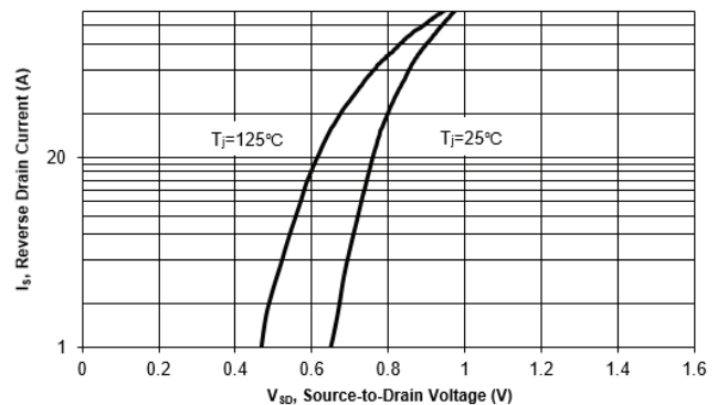
Fig. 6 Typical Body-Diode Forward Characteristics
