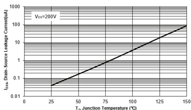
Fig. 8 Drain-Source Leakage Current vs. T_J
