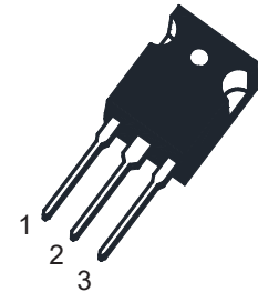
TO-247 Plastic Package 1.Gate 2.Drain 3.Source
