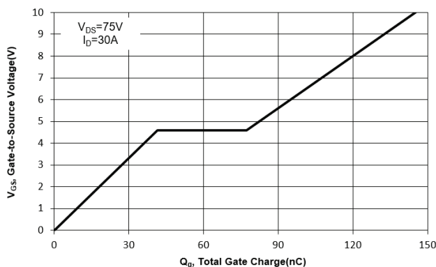
Fig. 11 Gate Charge
