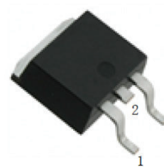
1.Gate 2.Drain 3.Source TO-252 Plastic Package
