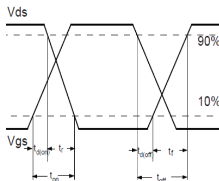
Fig.1-2 Switching Waveform
