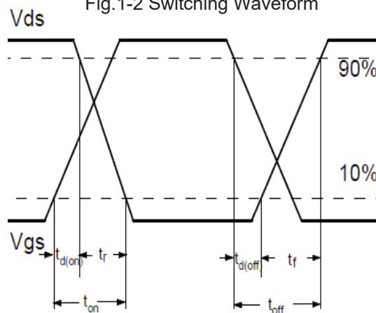
Fig.1-2 Switching Waveform
