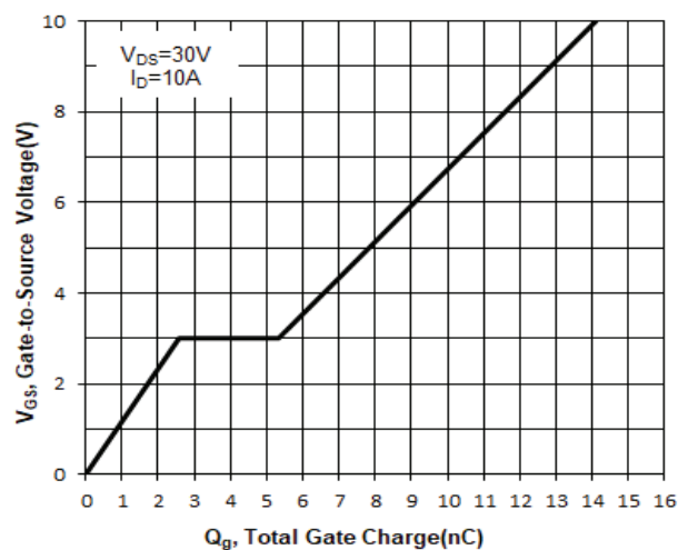
Fig 10. Gate Charge
