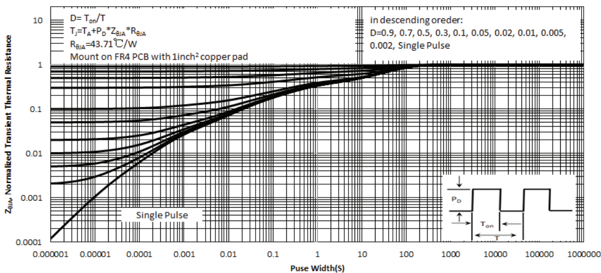
Fig. 13 Normalized Maximum Transient Thermal Impedance( z_{\theta JA} )
