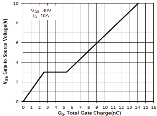
Fig. 10 Gate Charge
