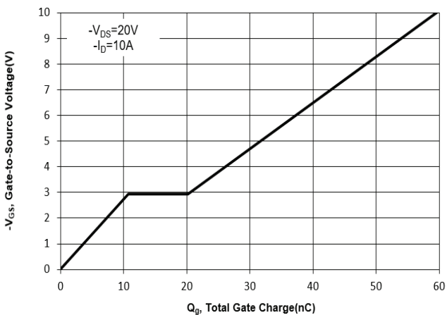
Fig. 11 Gate Charge
