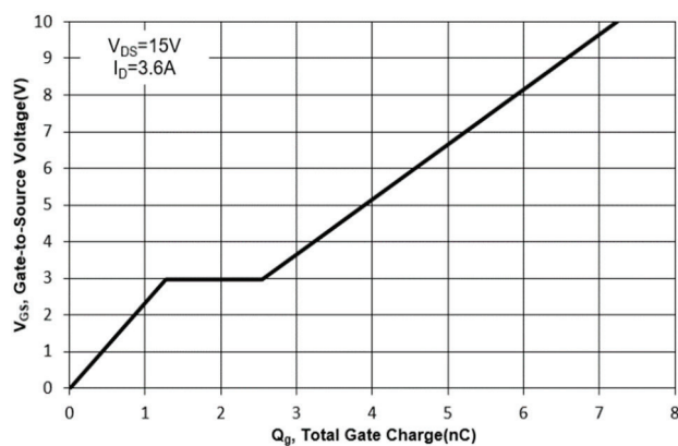
Fig. 11 Gate Charge
