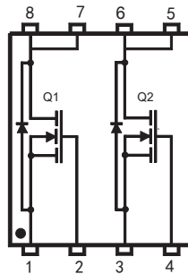
Q1:1.Source 2.Gate 7.Drain 8.Drain Q2:3.Source 4.Gate 5.Drain 6.Drain DFN3030 Plastic Package
