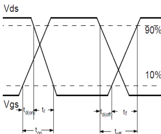
Fig.1-2 Switching Waveform
