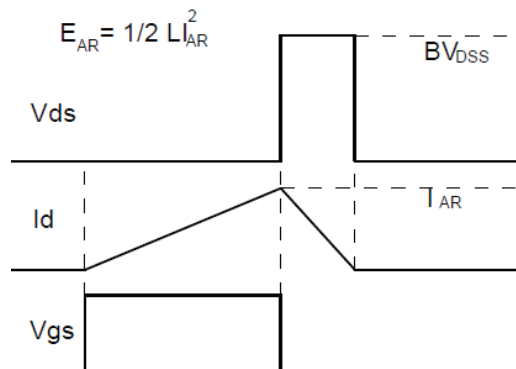
Fig.3-2 Avalanche waveform
