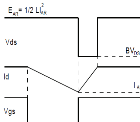
Fig.3-2 Avalanche waveform
