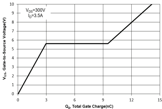
Fig. 11 Gate Charge
