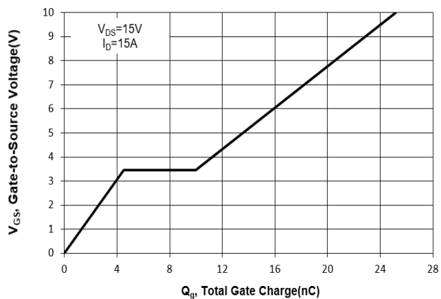
Fig. 11 Gate Charge
