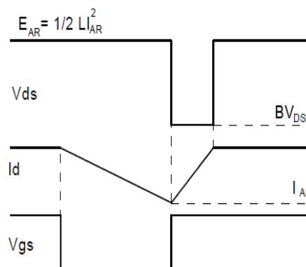
Fig.3-2 Avalanche waveform
