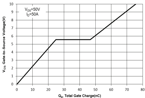
Fig. 11 Gate Charge
