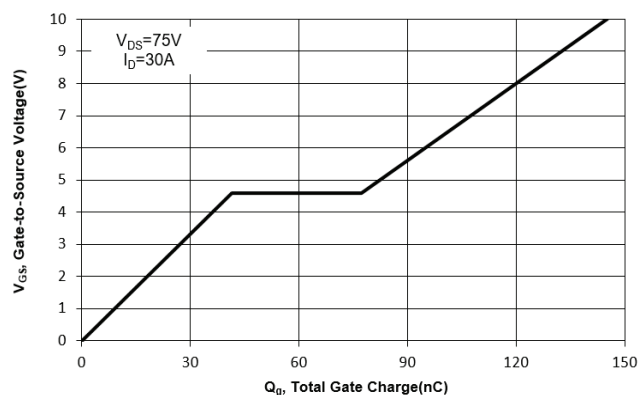
Fig. 11 Gate Charge
