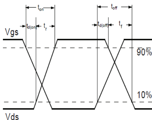
Fig.1-2 Switching Waveform
