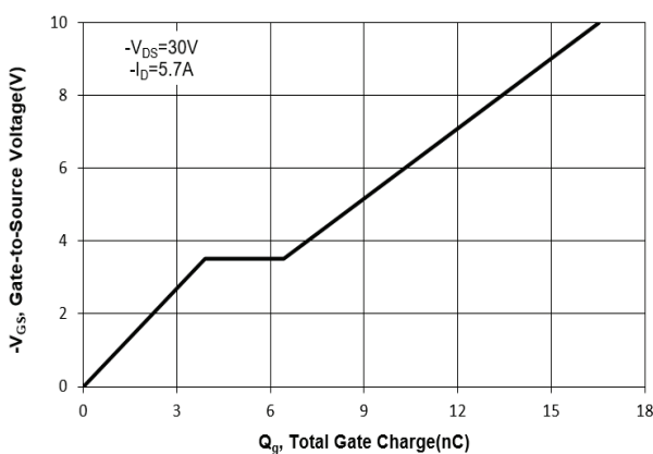
Fig. 11 Gate Charge
