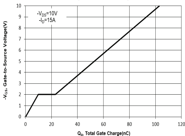
Fig. 11 Gate Charge
