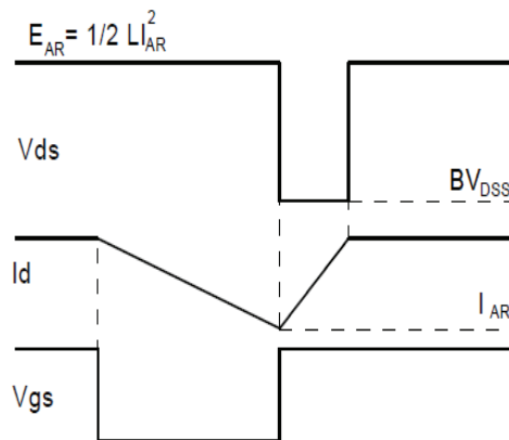
Fig.3-2 Avalanche waveform
