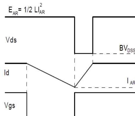
Fig.3-2 Avalanche waveform
