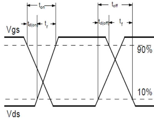
Fig.1-2 Switching Waveform
