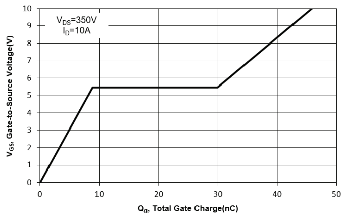
Fig. 11 Gate Charge
