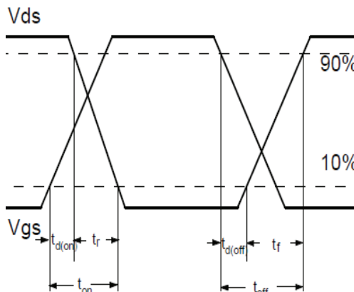
Fig.1-2 Switching Waveform
