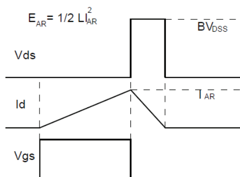
Fig.3-2 Avalanche waveform
