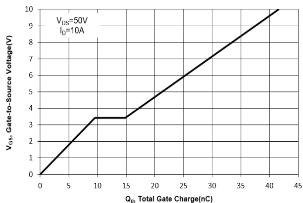
Fig. 11 Gate Charge
