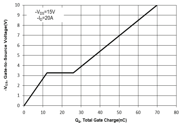
Fig. 11 Gate Charge
