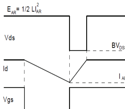
Fig.3-2 Avalanche waveform
