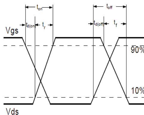
Fig.1-2 Switching Waveform
