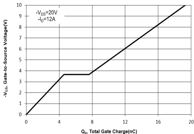
Fig. 11 Gate Charge
