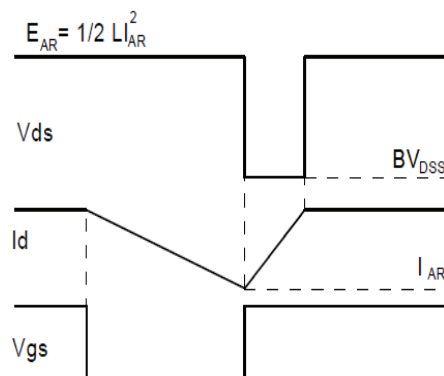
Fig.3-2 Avalanche waveform
