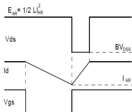
Fig.3-2 Avalanche waveform
