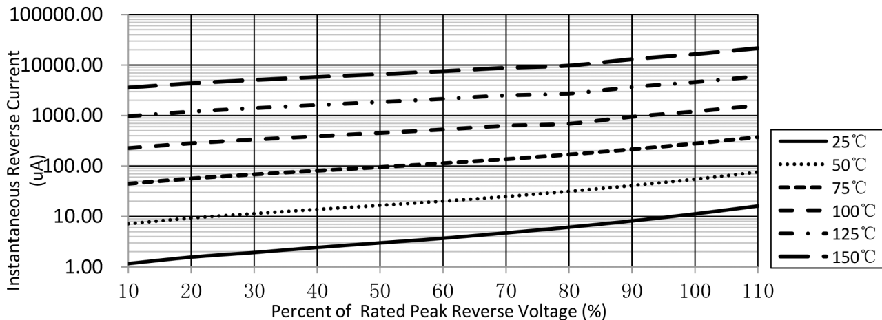
Figure 4. Typical Reverse Characteristics (SK32A thru SK34A)
