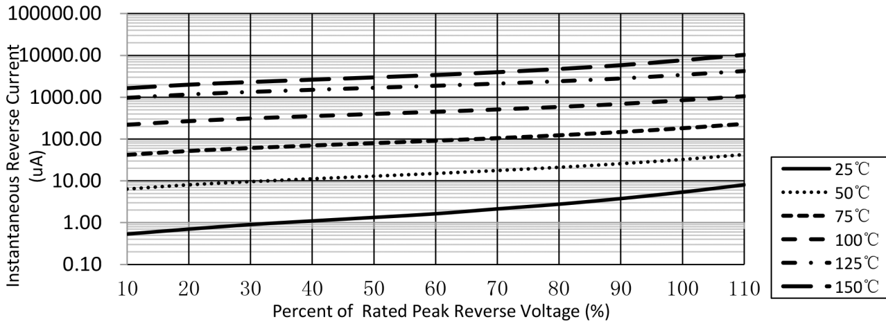
Figure 6. Typical Reverse Characteristics (SK35A thru SK36A)
