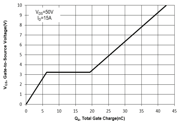
Fig. 11 Gate Charge
