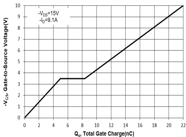
Fig. 11 Gate Charge
