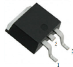
1.Gate 2.Drain 3.Source
