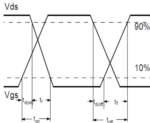
Fig.1-2 Switching Waveform
