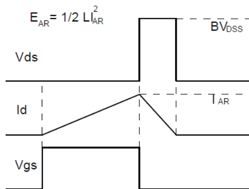
Fig.3-2 Avalanche waveform
