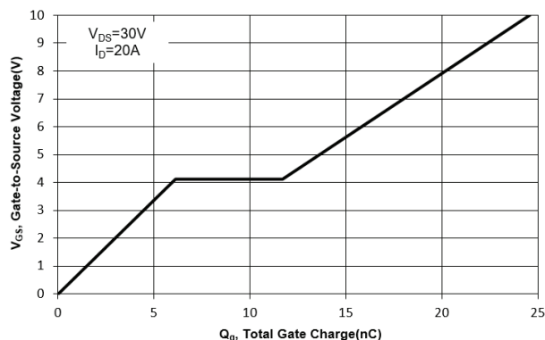
Fig. 11 Gate Charge
